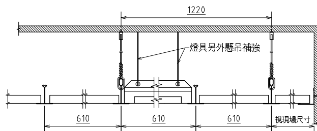
C-C SECTION
